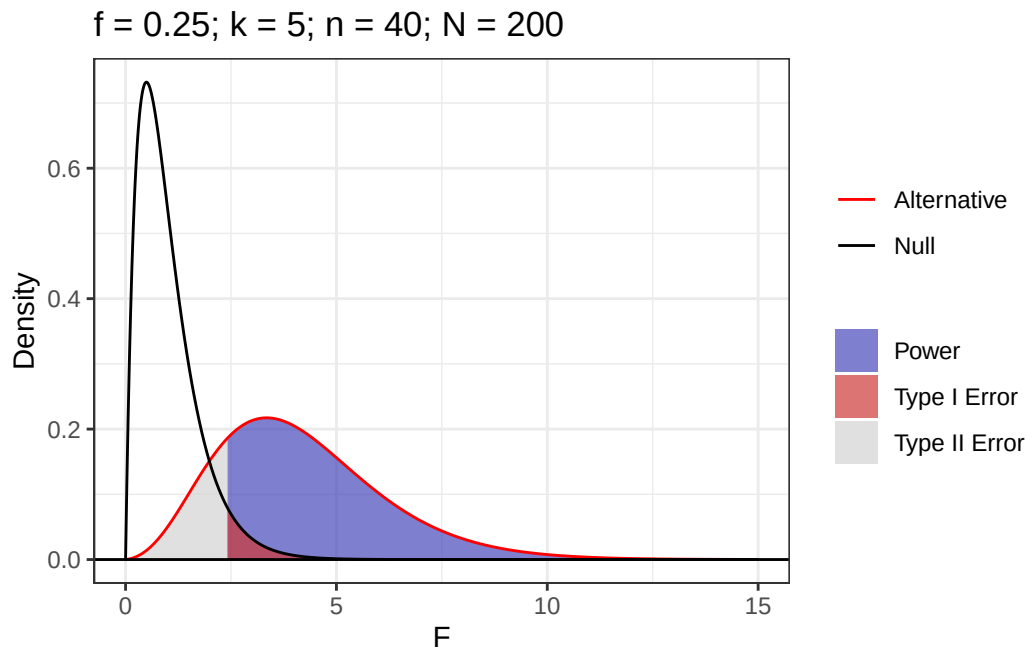
Figure 1: Power Analysis Of Minimally Powered Sample Size
