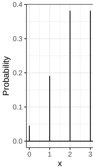
theta = 1
