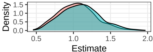
Exponential n = 20
