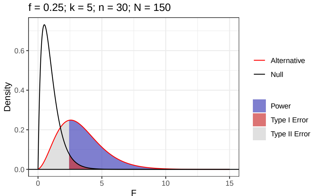
Figure 2: Power Analysis of Under Powered Sample Size
