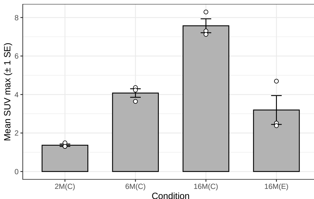
Figure 3: SUV max by Condition
