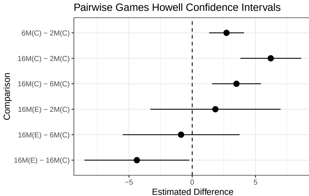
Figure 4: Post-Hoc Confidence Intervals
