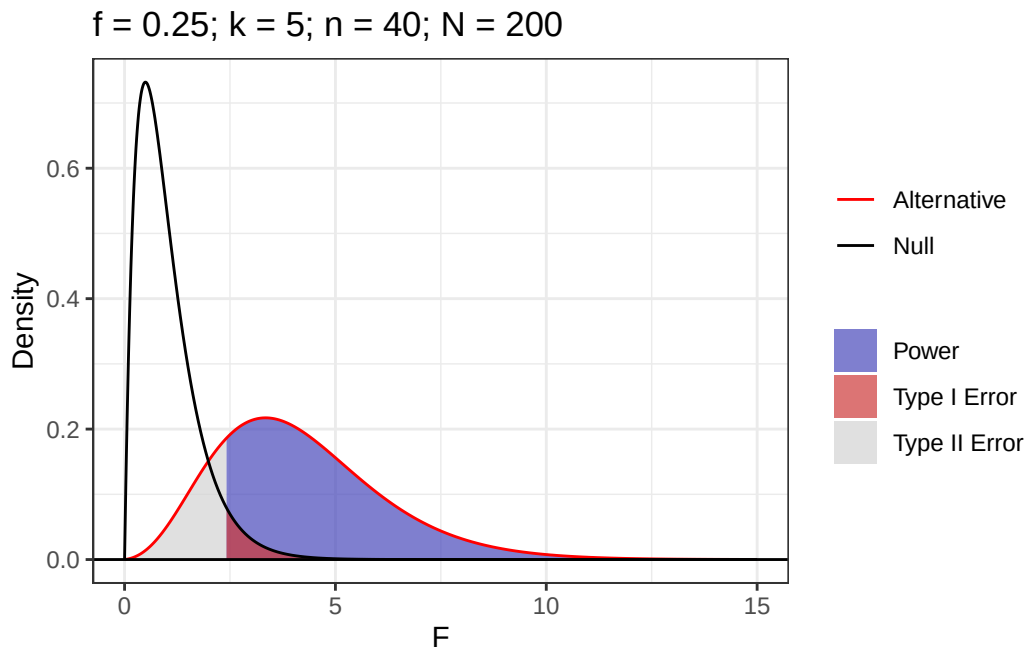
Figure 1: Power Analysis Of Minimally Powered Sample Size
