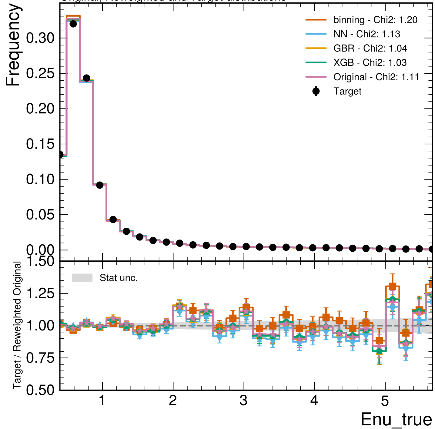
Original, Reweighted and Target distributions
