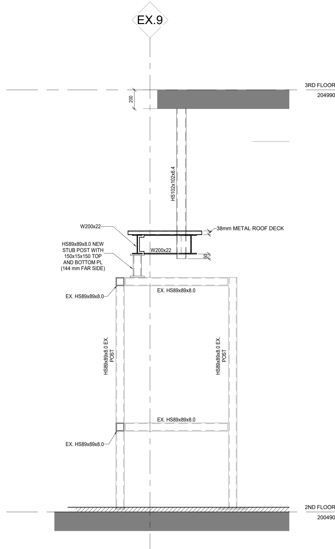
3 SECTION S401 1:20
