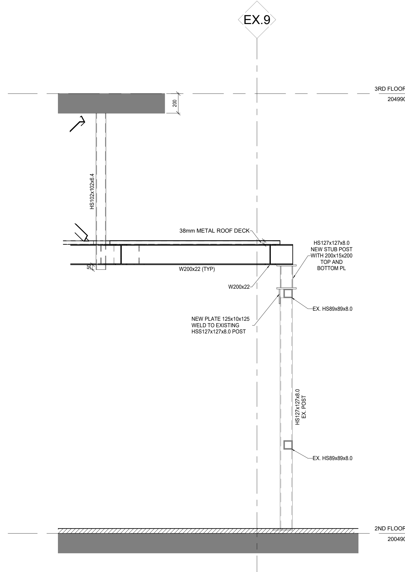
2 SECTION S401 1:20
