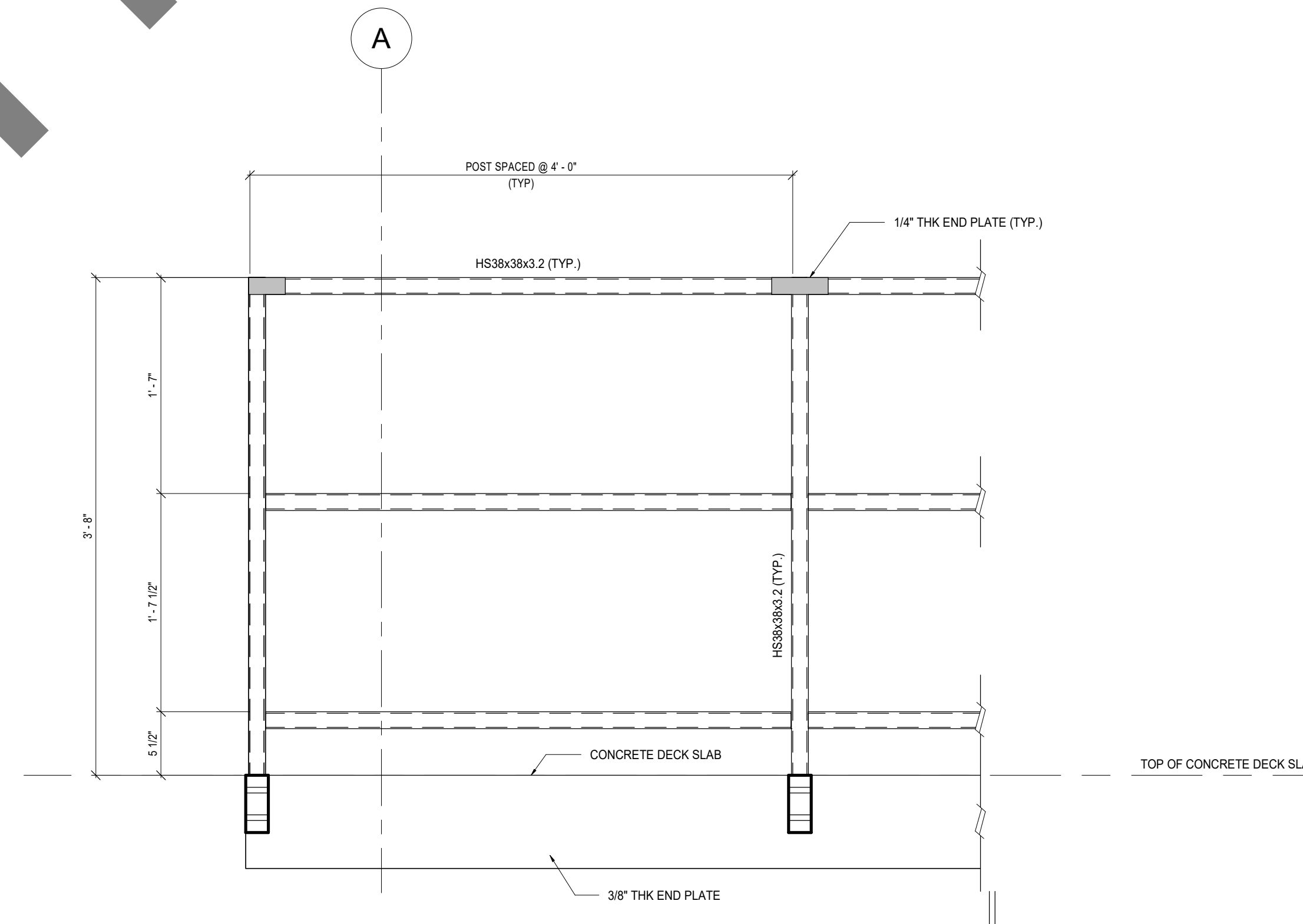
5 STEEL RAILING DETAILS S301 1:10
