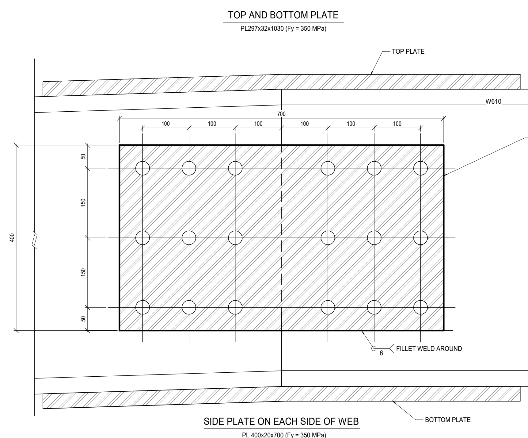
6 SPLICE CONNECTION PLATE DETAILS S301 1:5
