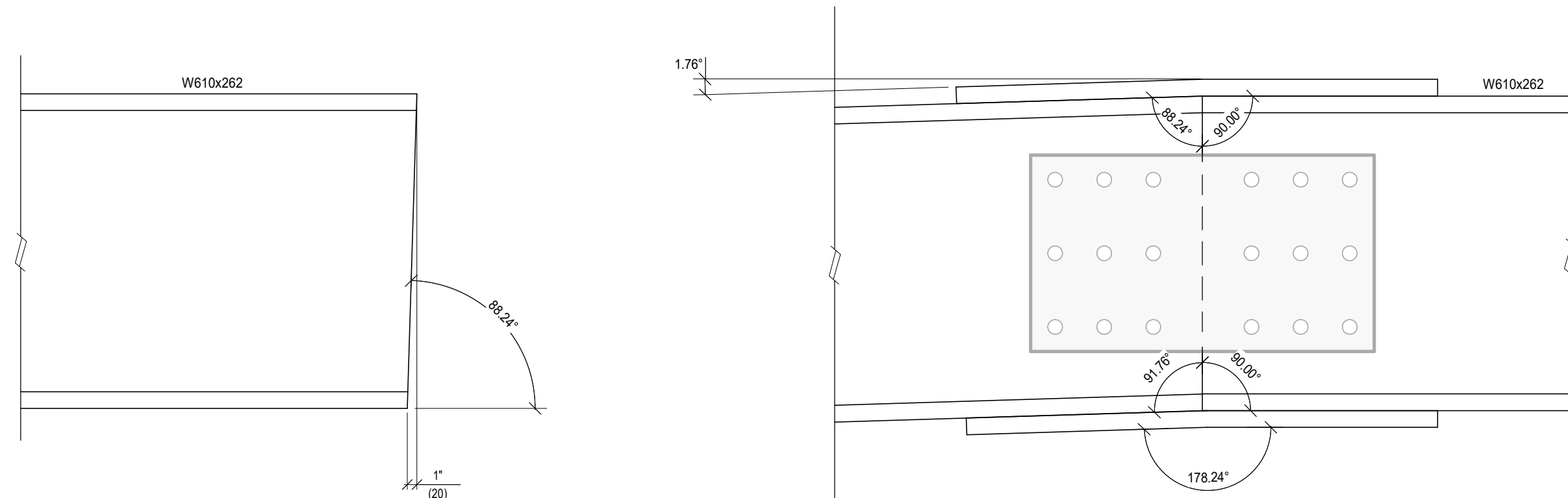
2 CUT DETAIL S302 1:10
