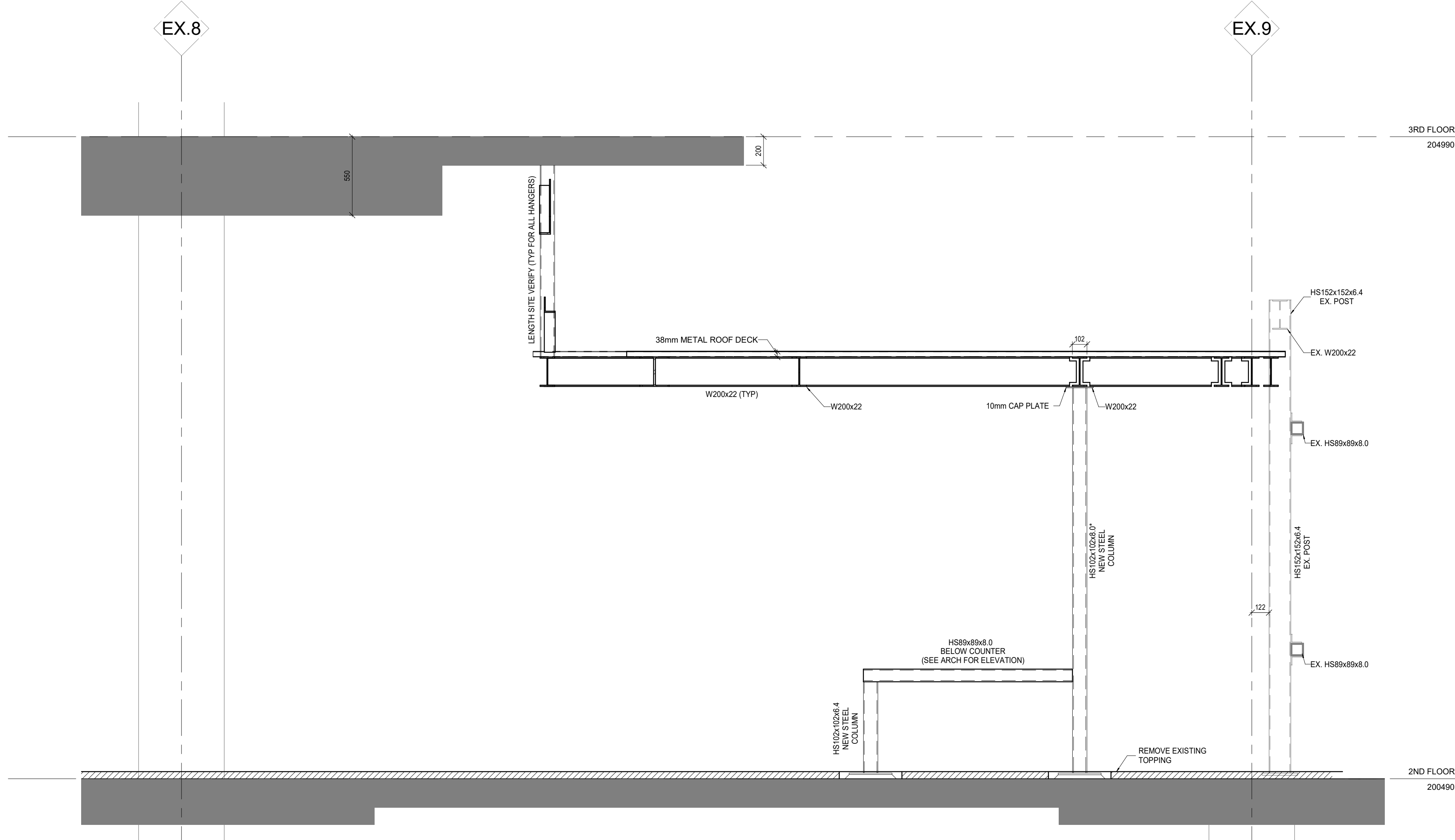
1 SECTION S401/ 1:20
