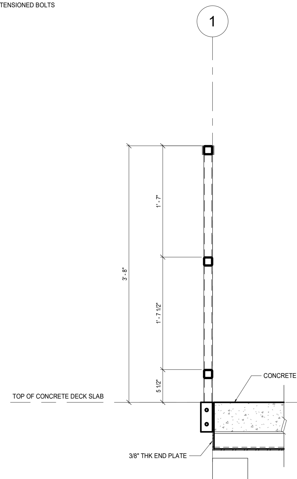
4 SECTION S301 1:10
