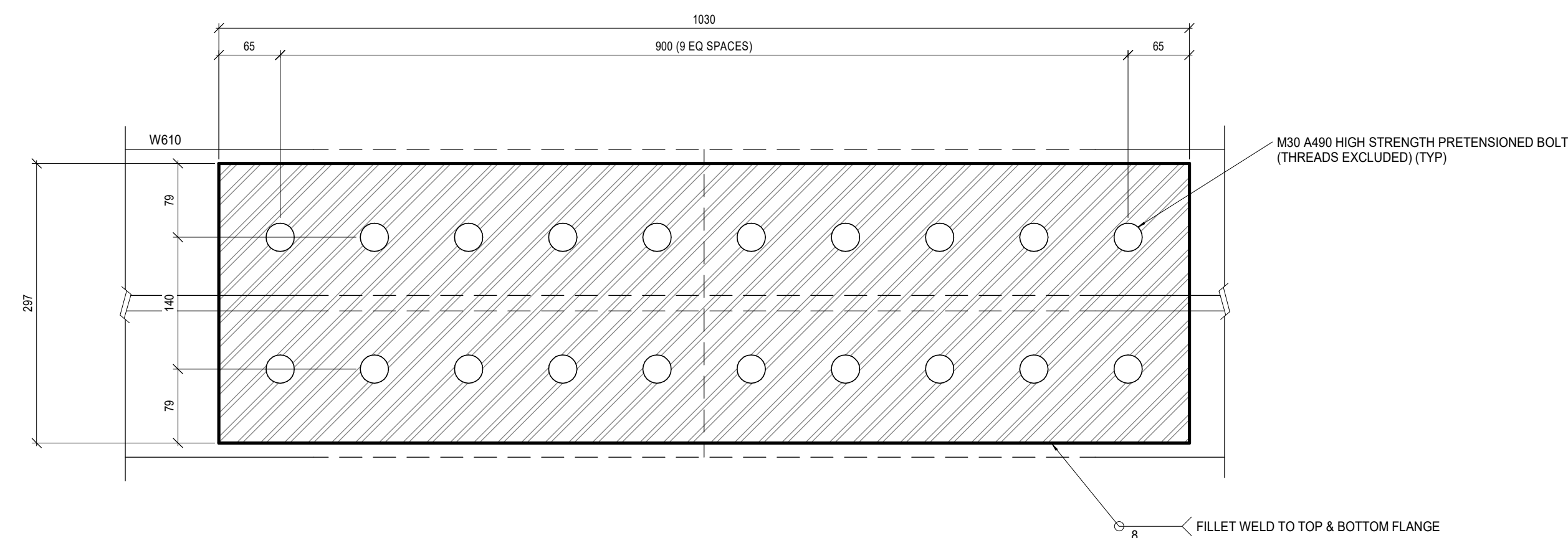
TOP AND BOTTOM PLATE PL 307x20x1030 (Fy = 50 MPa)
