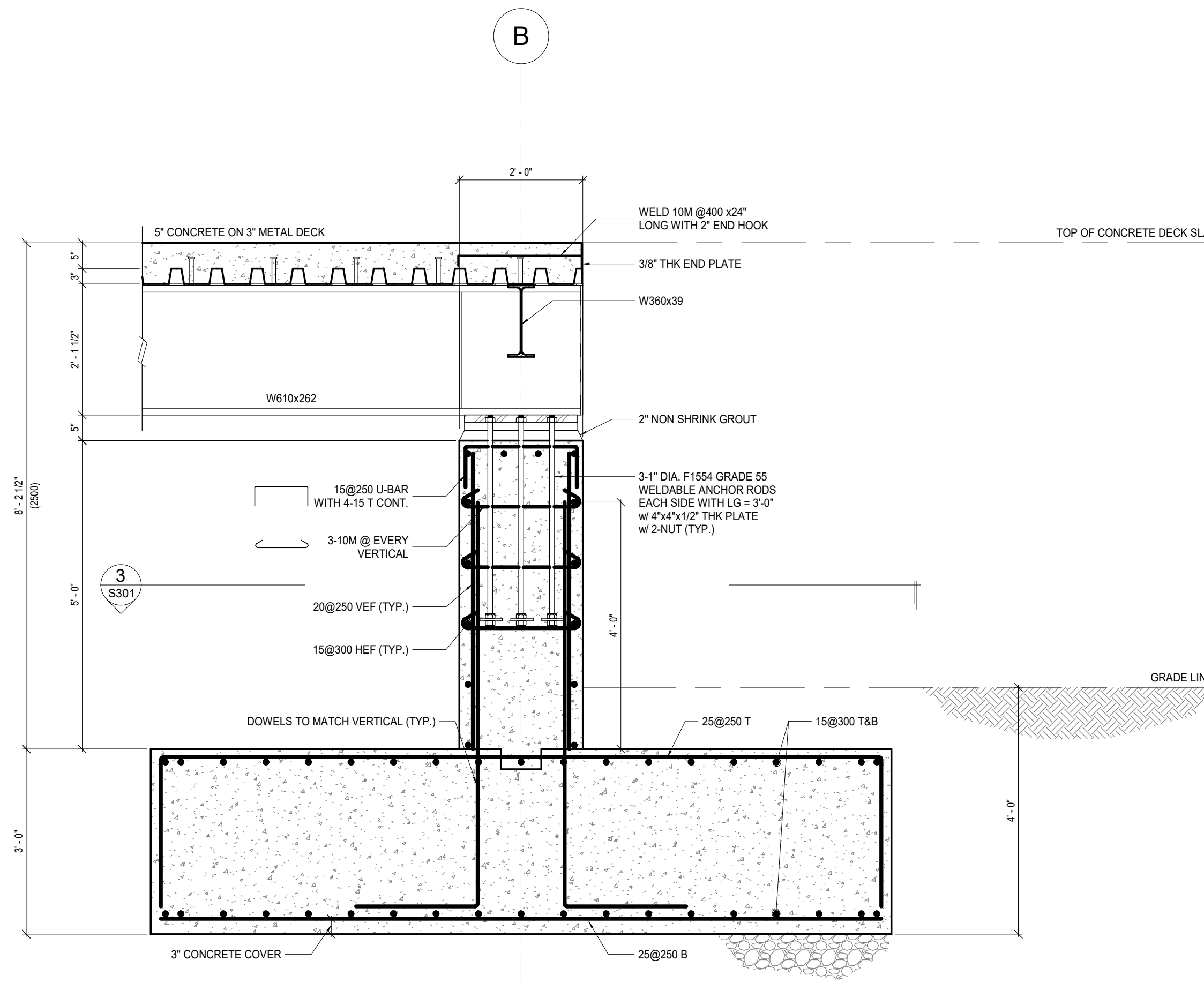
2 SLIDING END CONNECTION S301 1:20
