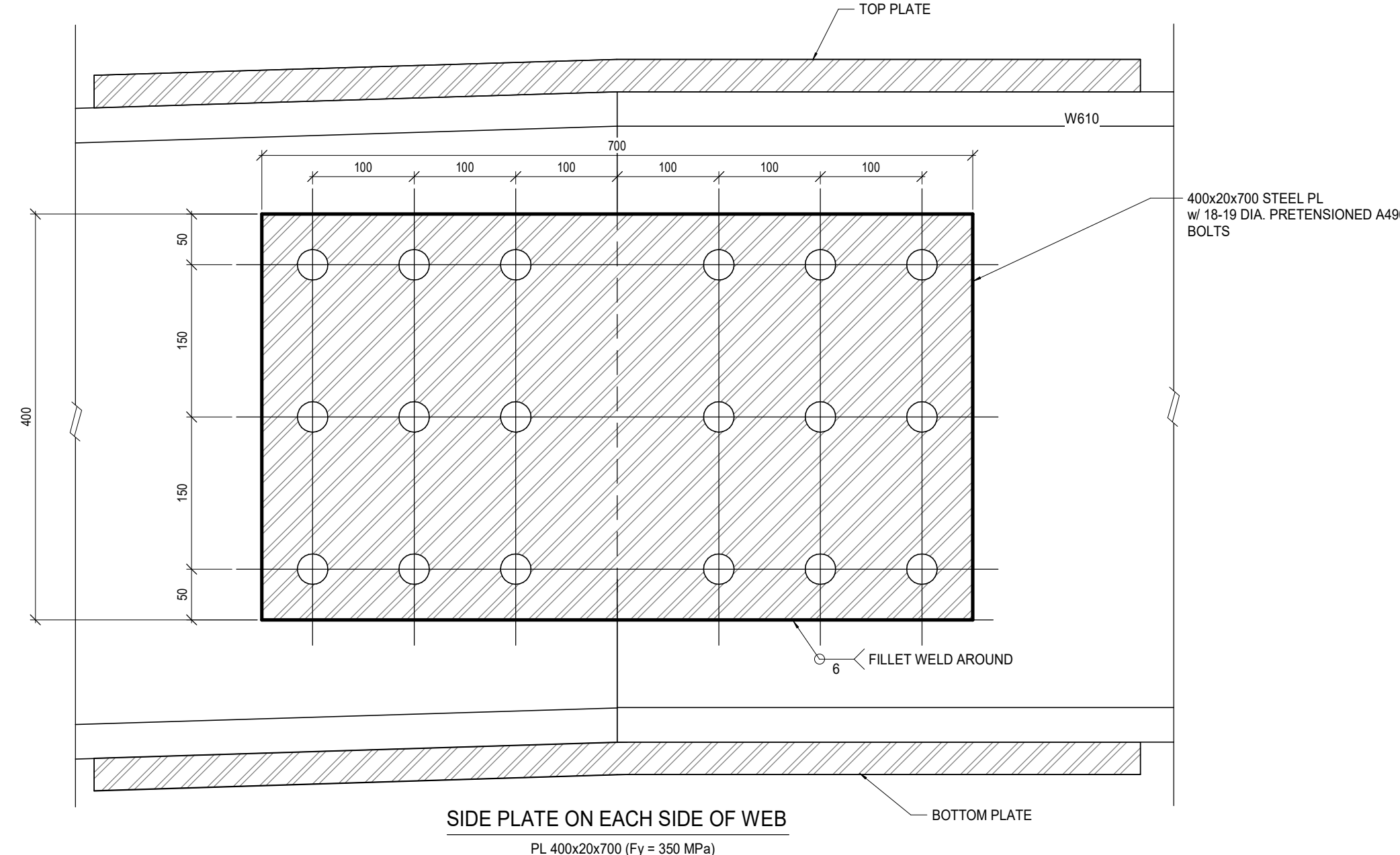
6 SPLICE CONNECTION PLATE DETAILS S301 1:5
