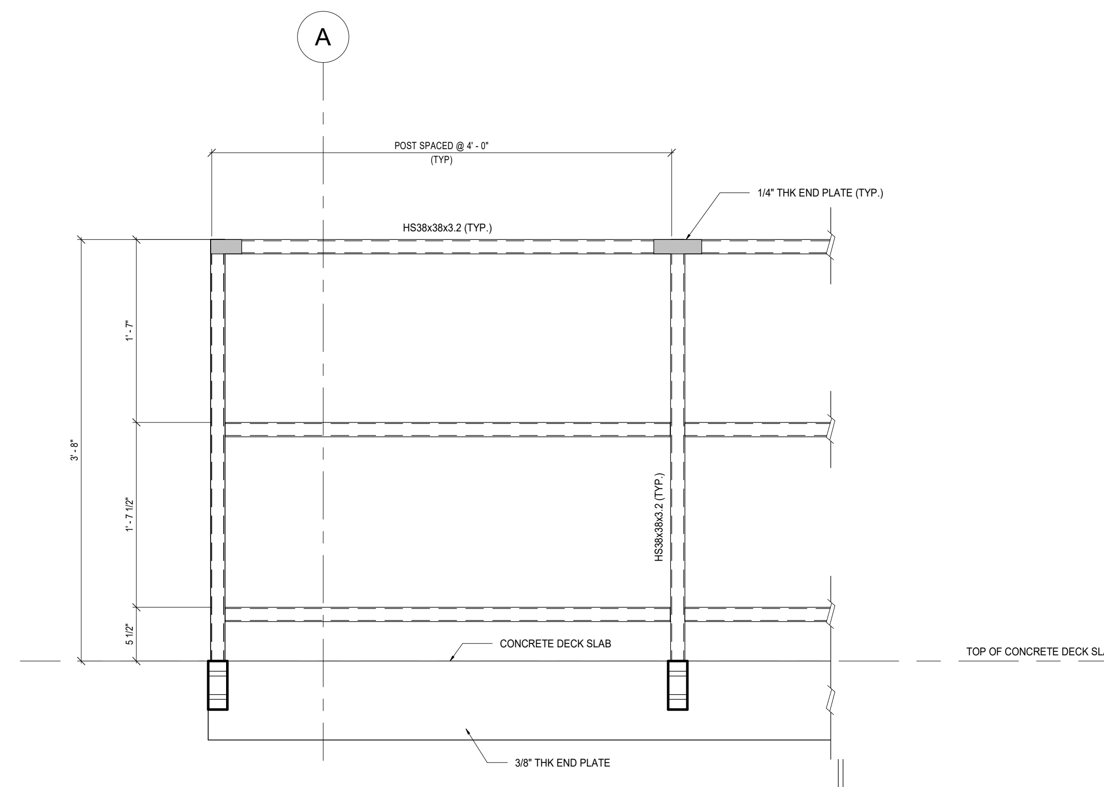
5 STEEL RAILING DETAILS S301 1:10
