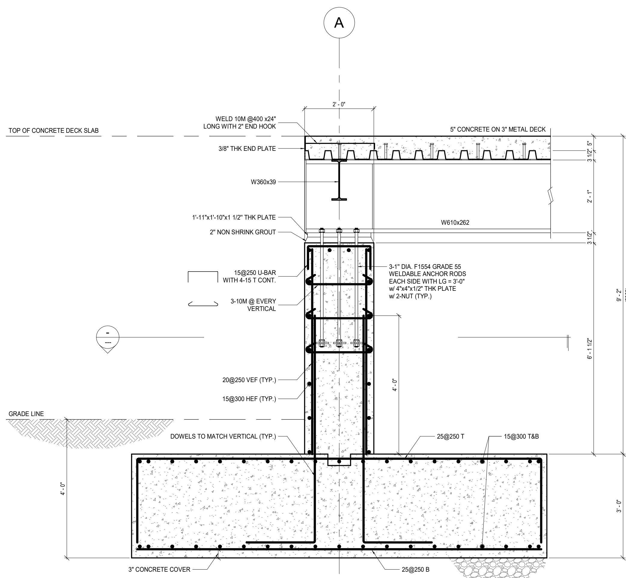
1 FIXED END CONNECTION S301 1:20
