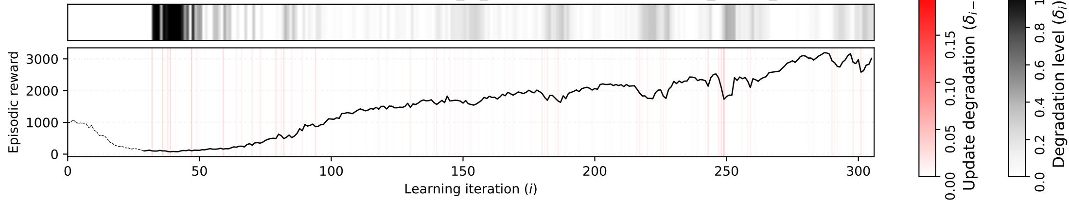
Degradation evolution (global: worsening_to_improvement; local: relative_reward_diff)
