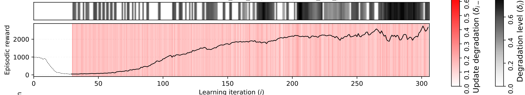
Degradation evolution (global: best_last_deg; local: paired_diff_probpos)
