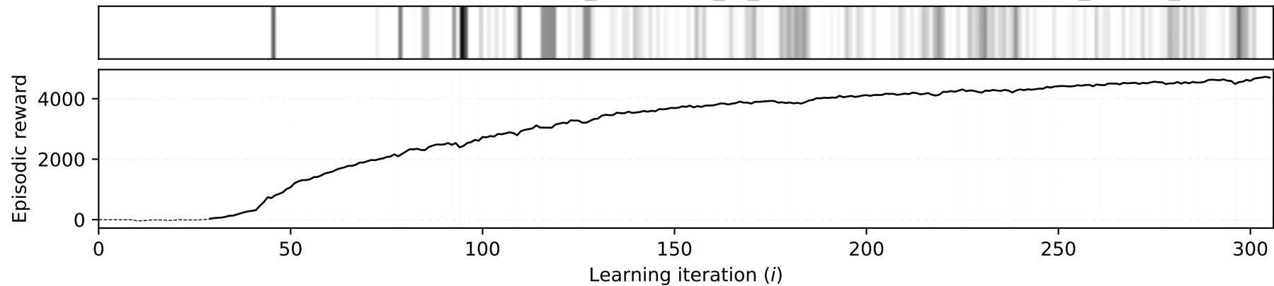
Degradation evolution (global: relative_worsening_to_improvement; local: relative_reward_diff)
