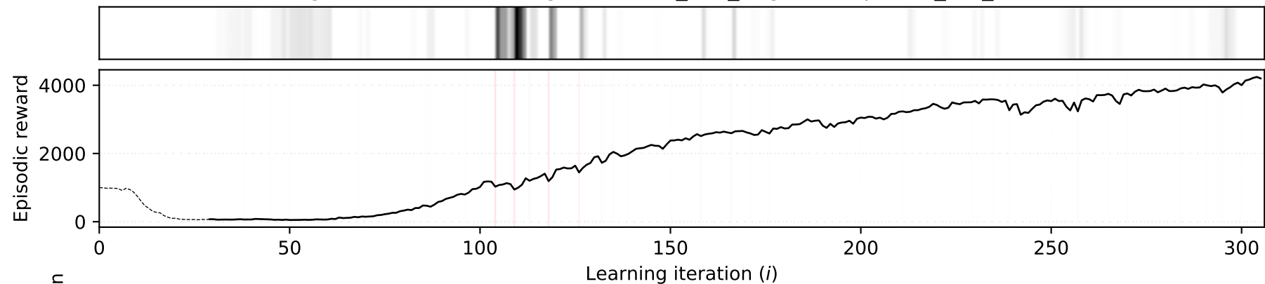
Degradation evolution (global: best_last_deg; local: paired_diff_median)
