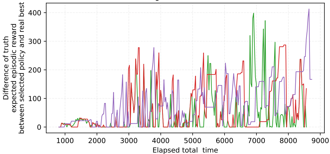
Magnitude evolution
