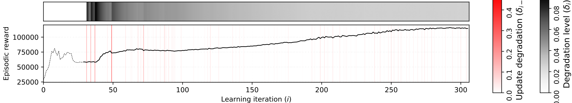
Degradation evolution (global: mean_update_deg; local: greater_prob)
