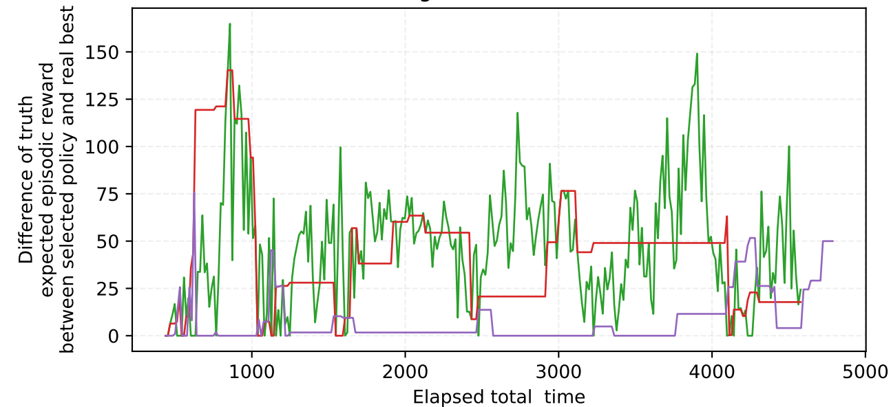
Magnitude evolution
