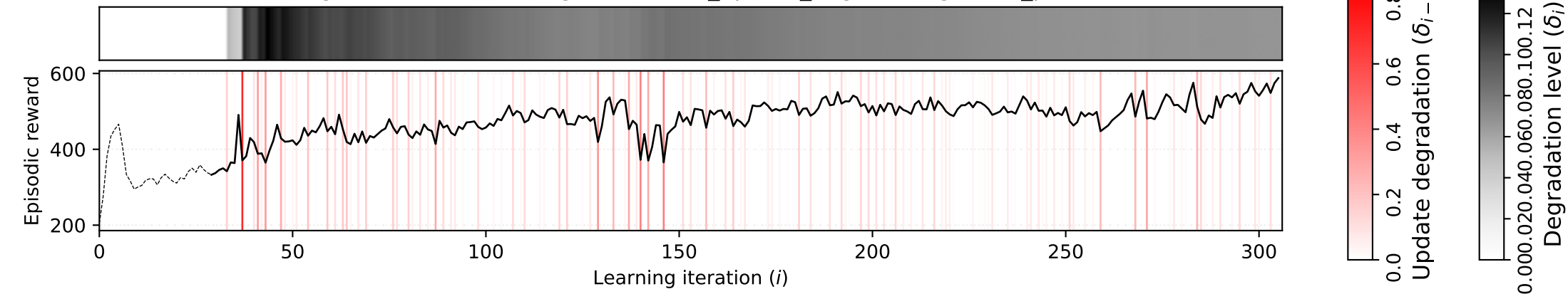
Degradation evolution (global: mean_update_deg; local: greater_prob)
