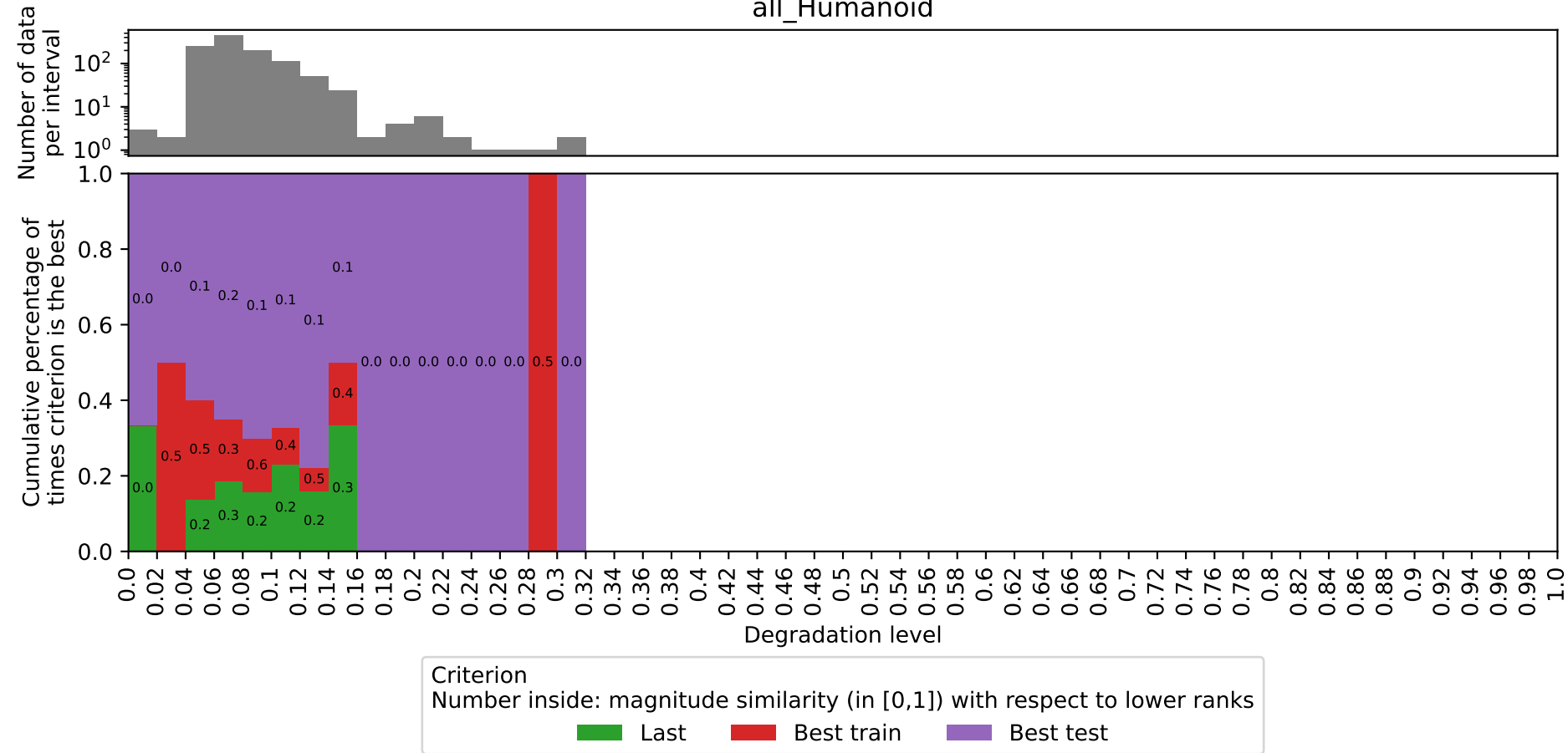
all_Humanoid
