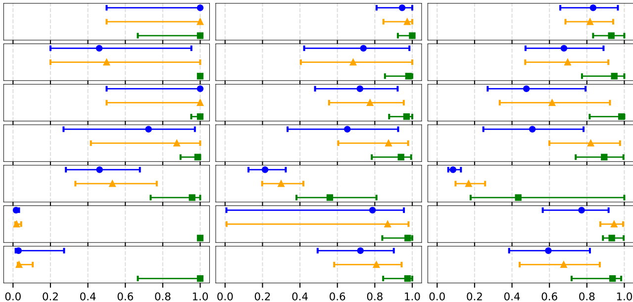
Learning
