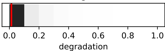
Learning (2068)
