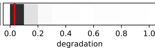
Stabilization (422)
