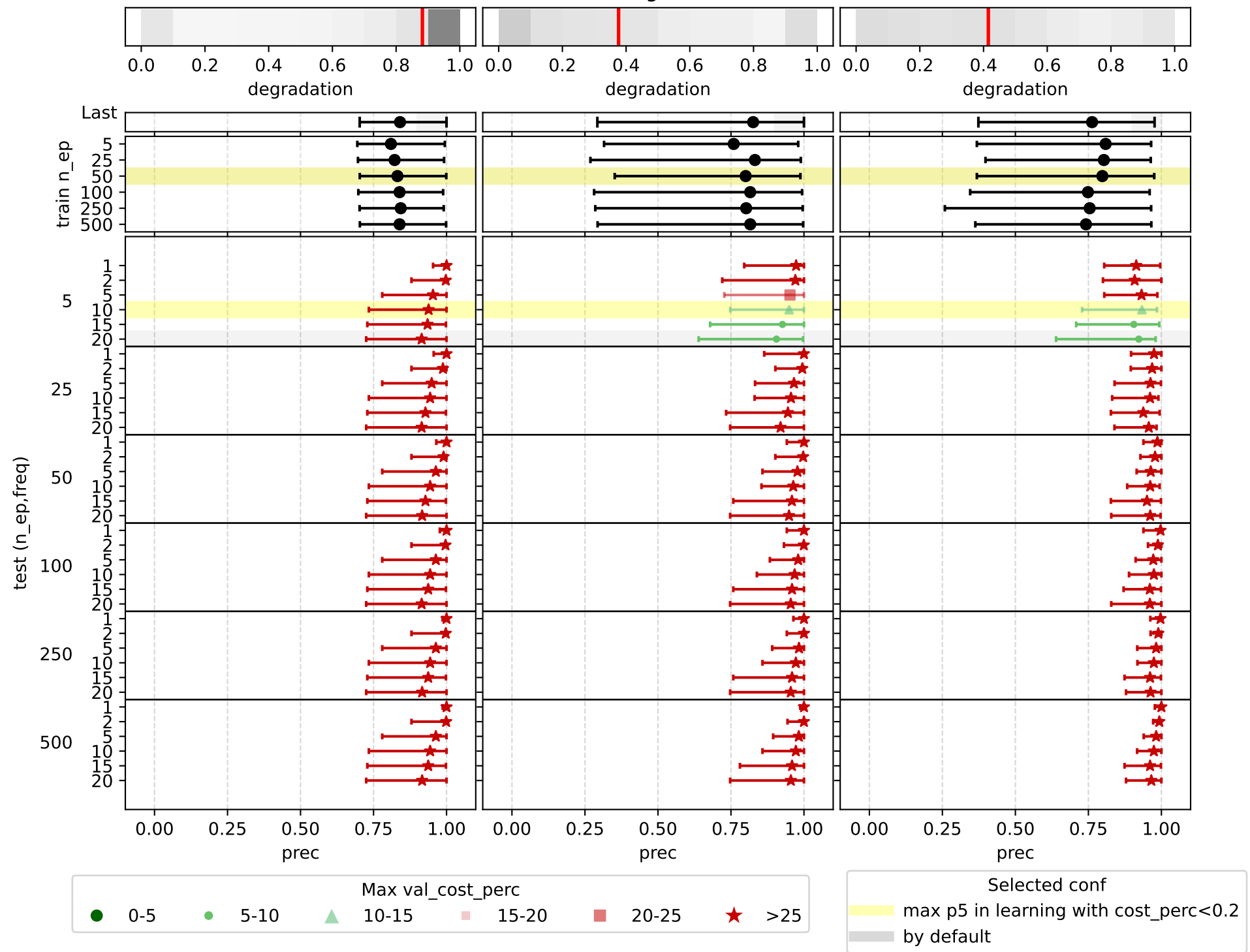
Initialization (4395)
