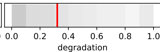
Stabilization (4467)
