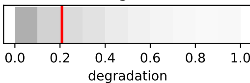
Learning (13878)
