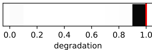
Initialization (3645)
