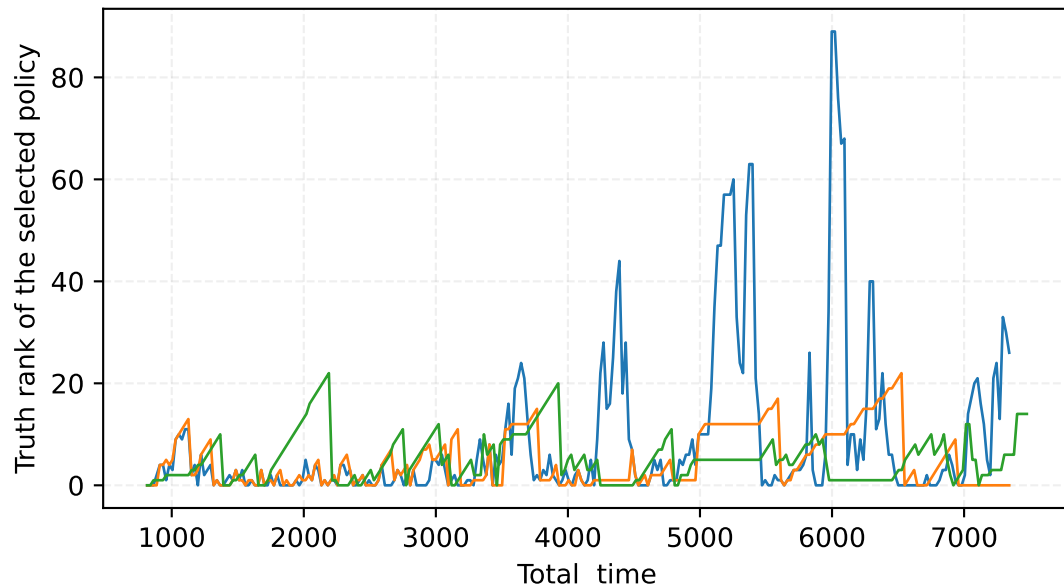
Rank evolution
