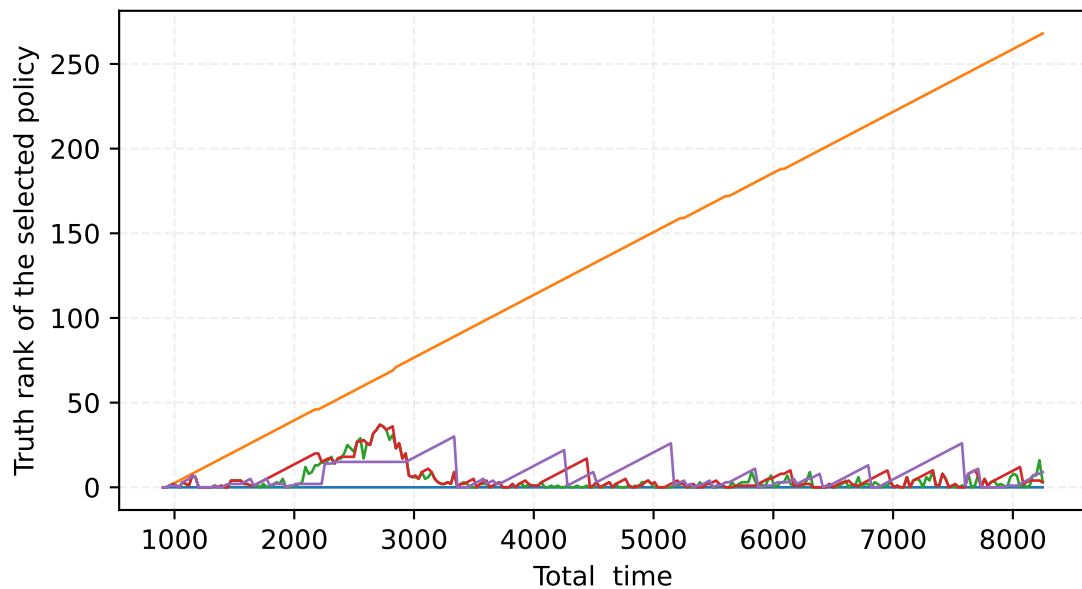
Rank evolution
