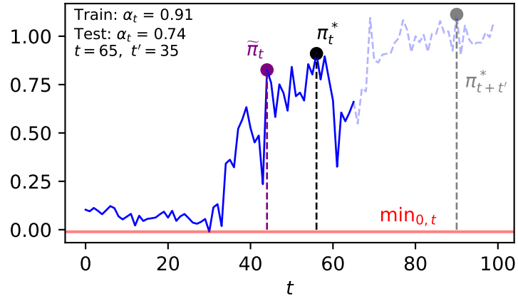
Accuracy
