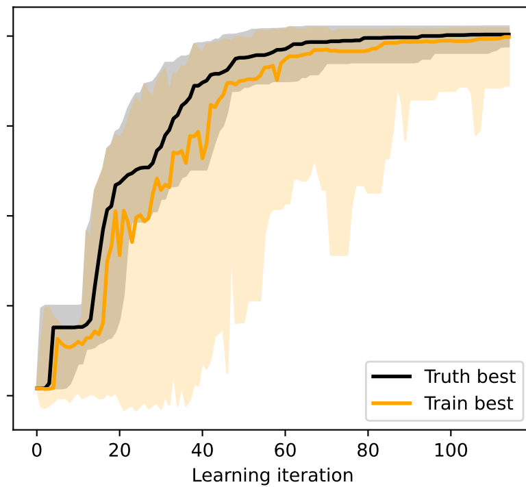
Truth vs default Train
