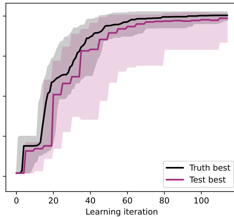
Truth vs default Test
