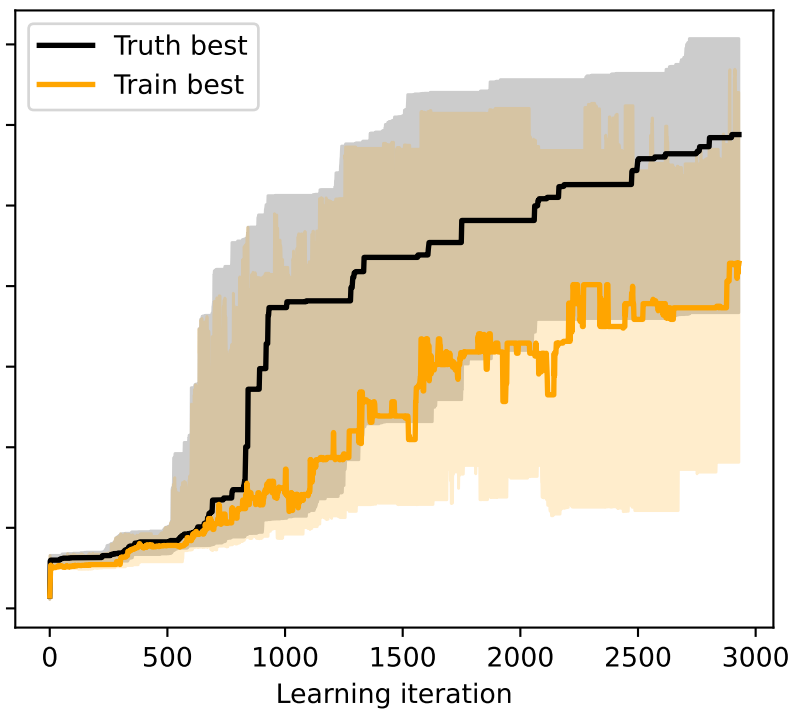
Truth vs default Train
