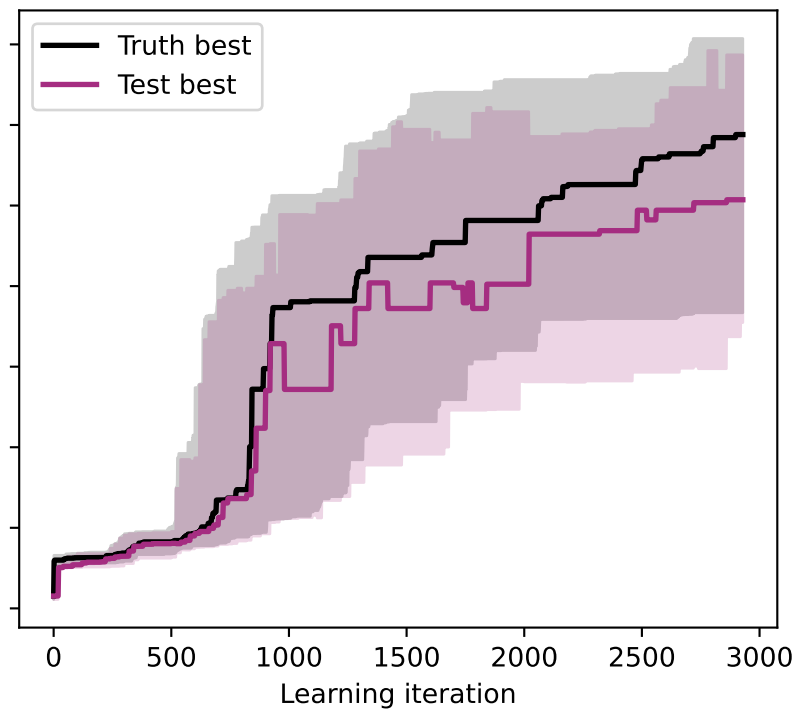
Truth vs default Test
