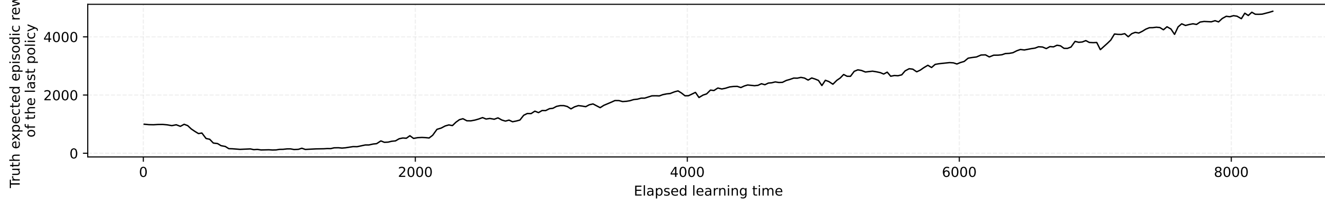
Learning-curve
