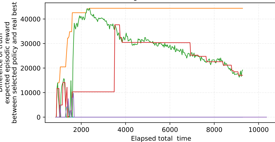
Magnitude evolution
