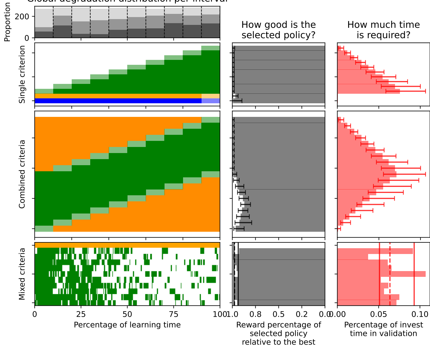
Global degradation distribution per interval
