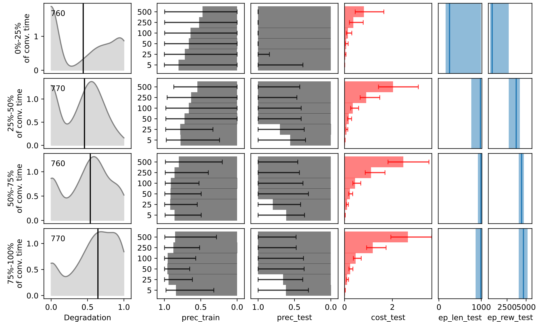
Walker2d
