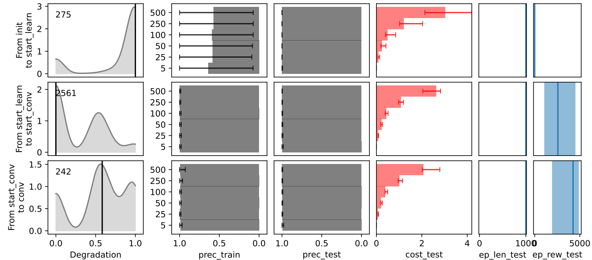
HalfCheetah
