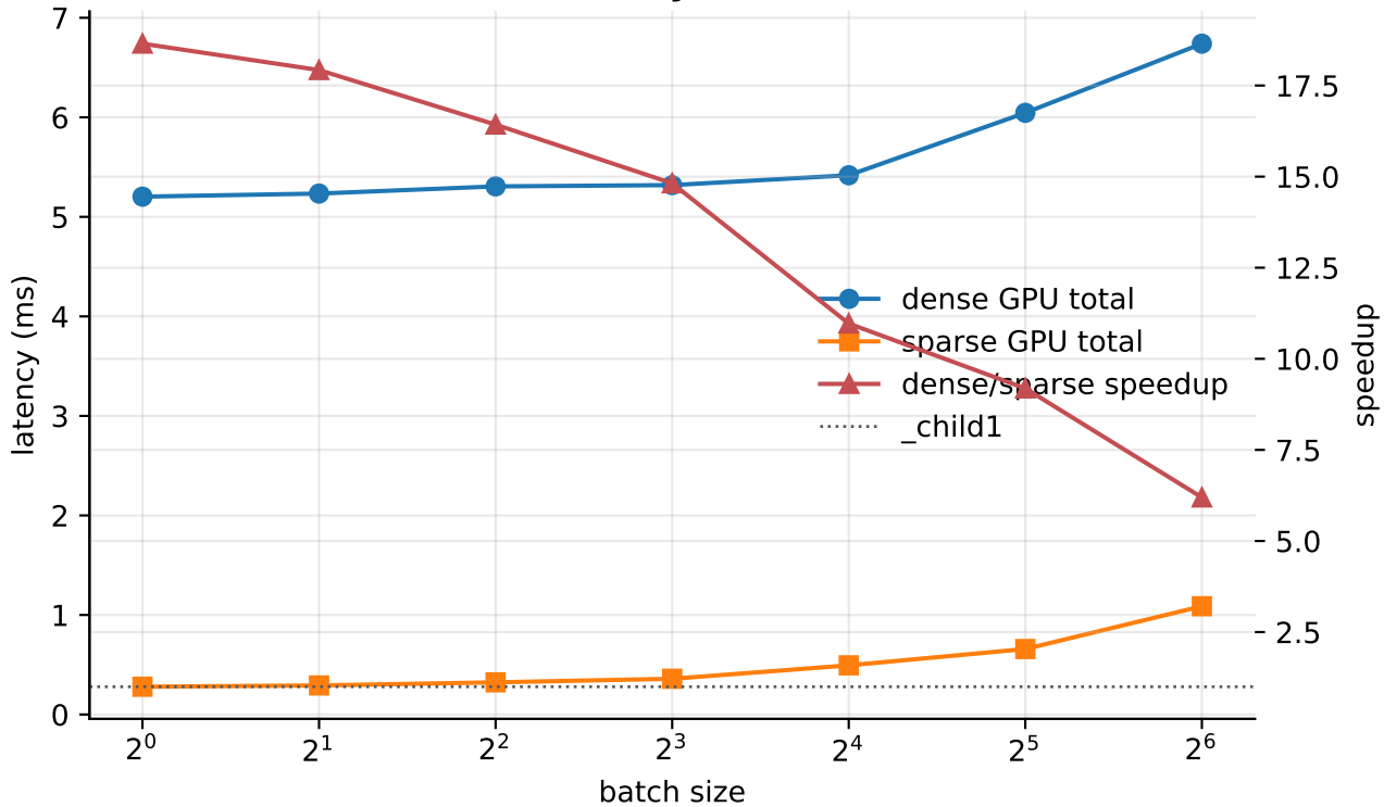
Decode Latency vs Batch Size
