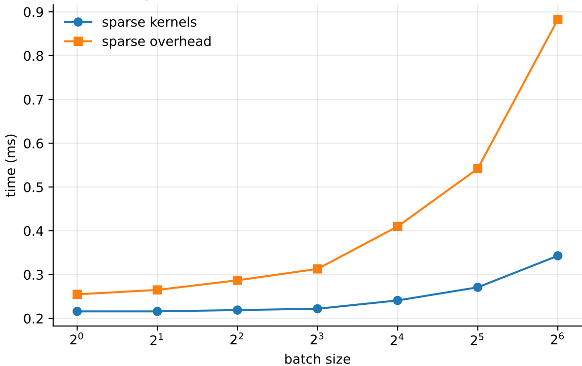
Sparse Runtime Breakdown vs Batch Size
