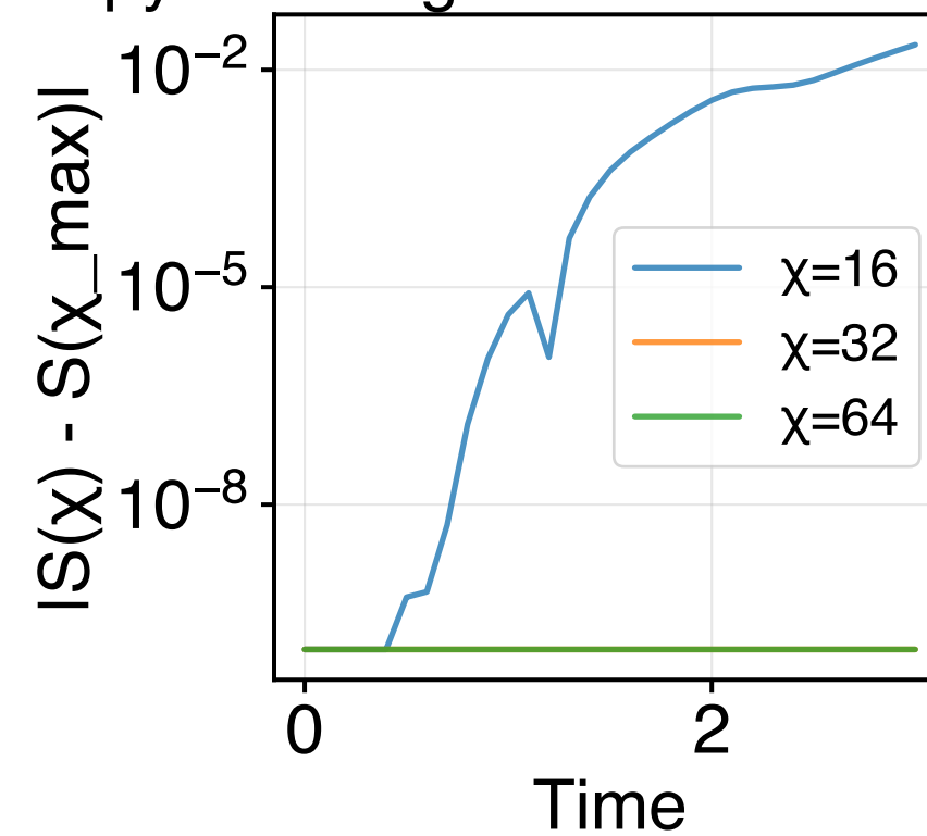
MPS Approximation Error
