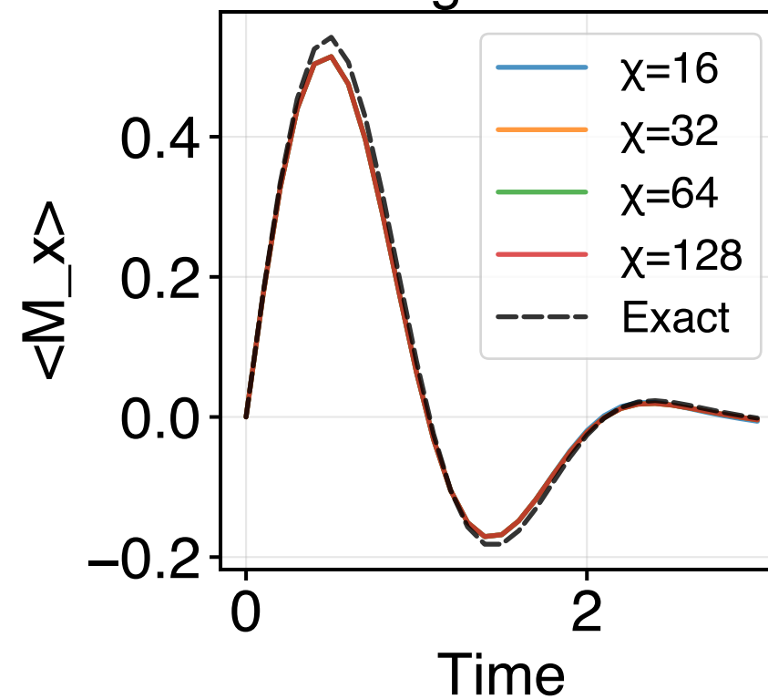
X-Magnetization
