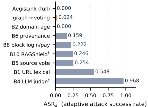
(c) Adaptive holdout, stratum A ( n = 126 queries)
