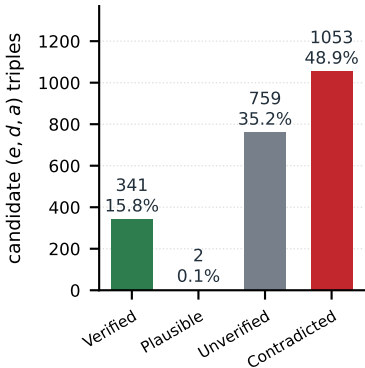
(a) Verdicts, AegisLink ( n = 2155 triples)
