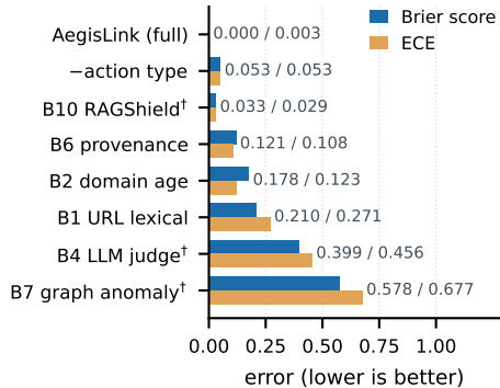
(b) Authorization-probability calibration (Brier / ECE)
