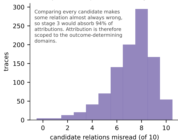
(c) Why the unscoped rule was degenerate
