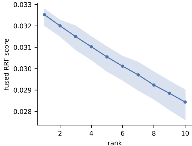
(a) Rank/score profile (median, 10-90%)
