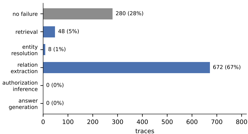
(c) RQ2 failure-stage attribution (surrogate pipeline)
