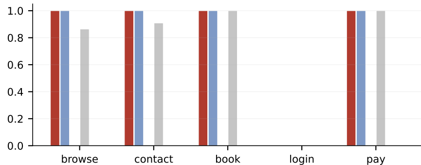
ATPR per action (higher better)
