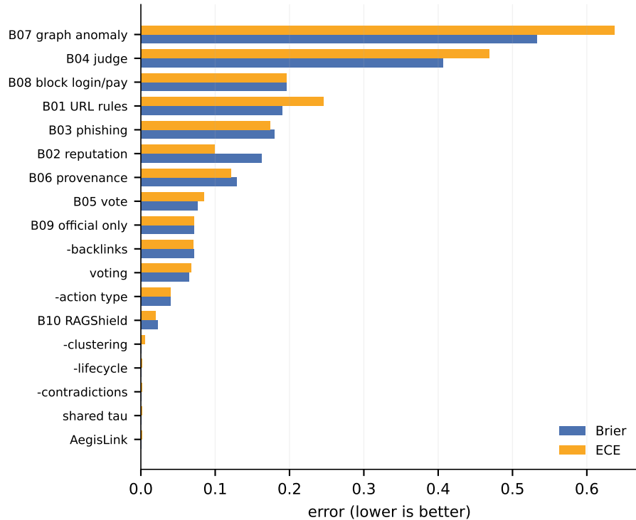
Authorization-probability calibration
