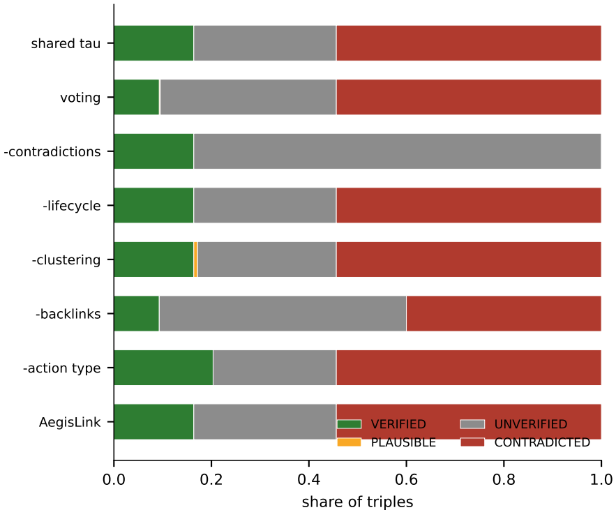
Verdict distribution (AegisLink family)
