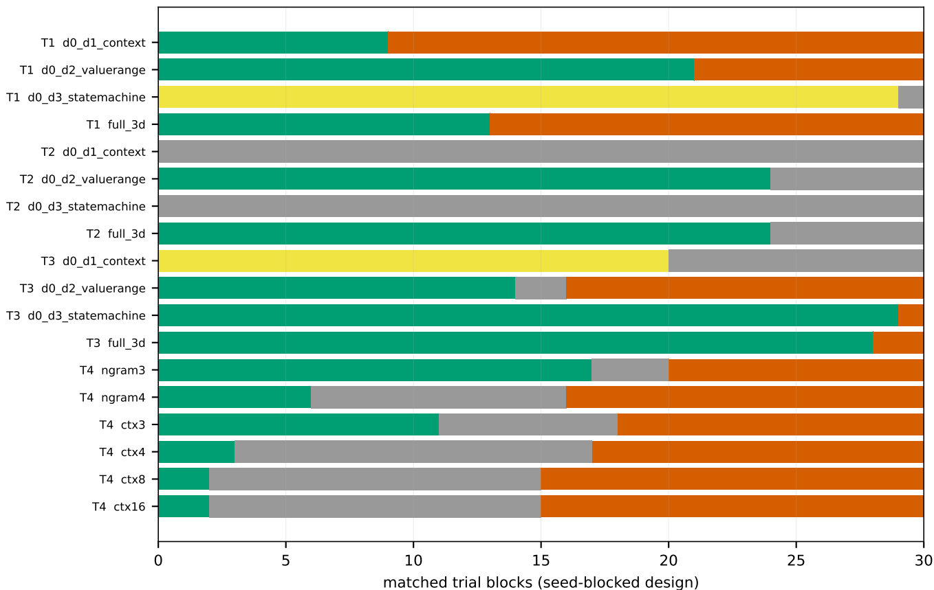
Trial-level paired outcomes against the edge-coverage control
