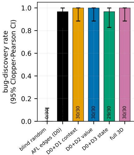
T1_context (budget 60,000 execs)
