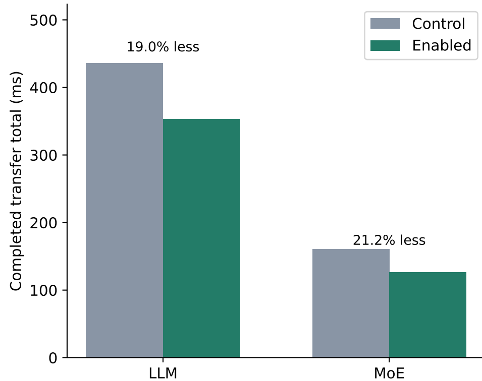
Dense upload: remove Sym staging copy
