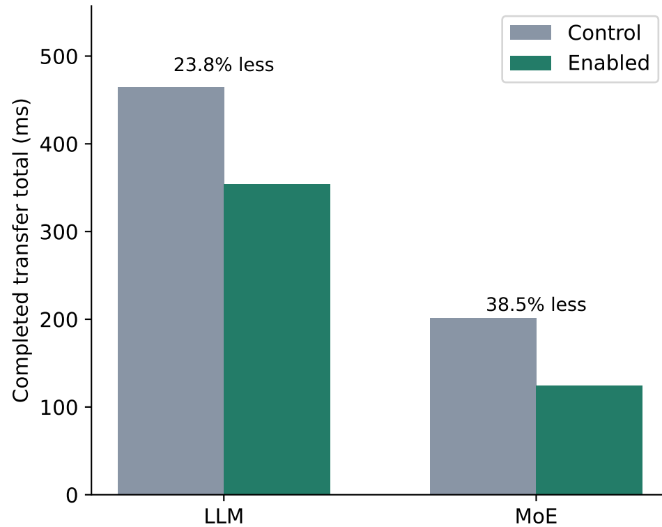
Direct calls: retain execution resources
