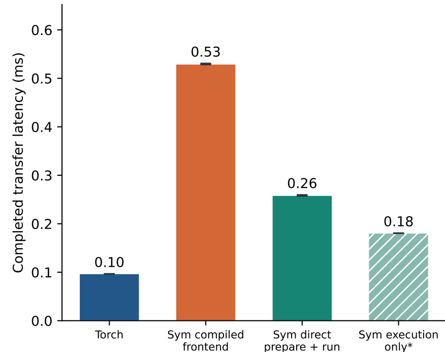
128 KiB KV eviction (D2H)
