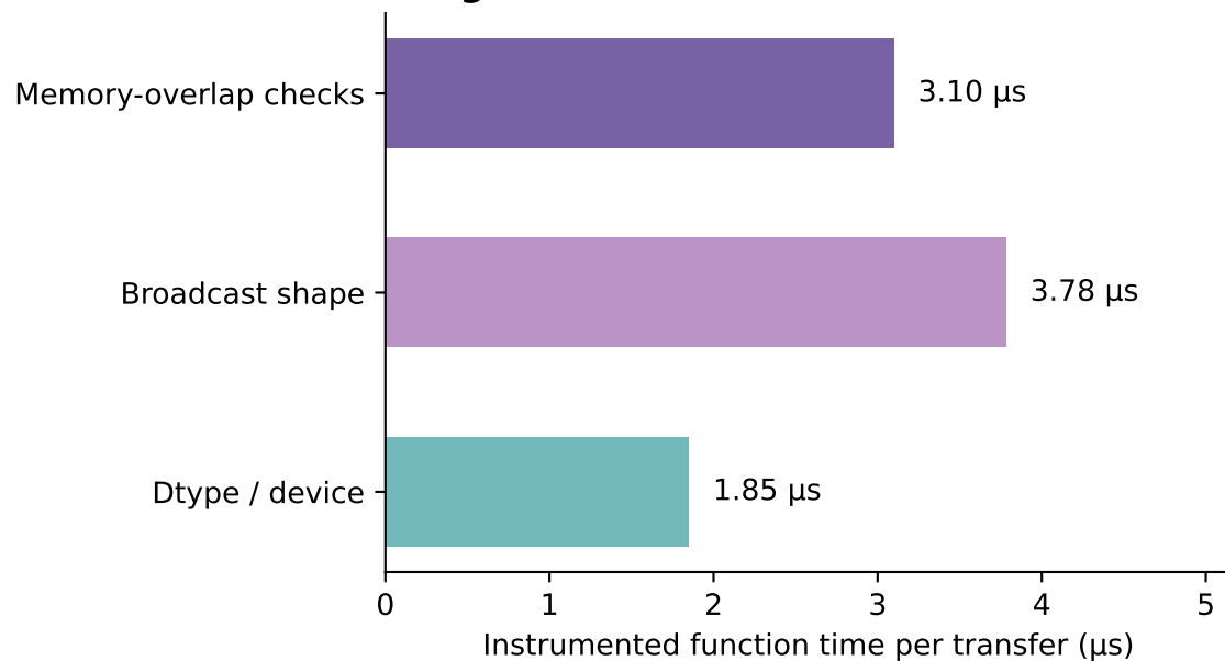
LLM weight fetch: 5 TensorIterator builds / transfer
