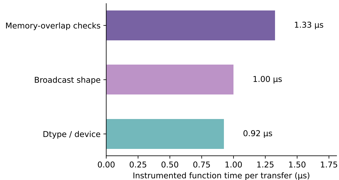
KV restore: 2 TensorIterator builds / transfer
