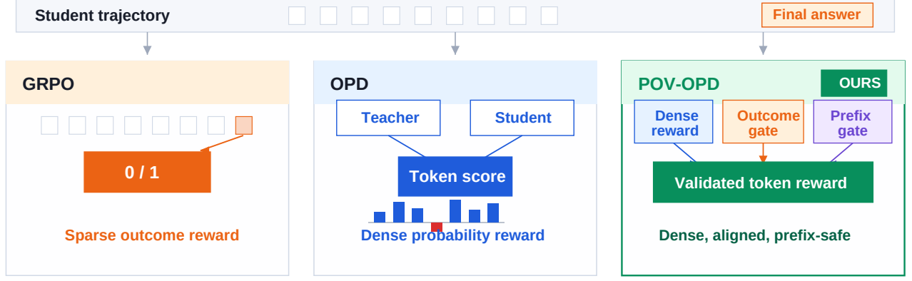
Figure 1: Reward estimators for the same student trajectory. GRPO provides only a terminal 0/1 outcome reward, whereas OPD derives dense token rewards from teacher–student probability differences. POV-OPD retains this dense signal while adding outcome validation and prefix-window gating, producing outcome-aligned, prefix-constrained token rewards.
