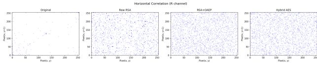
Figure 5: Correlation scatter (R, horizontal): original shows strong linear relationship; encrypted images show uniform scatter.
