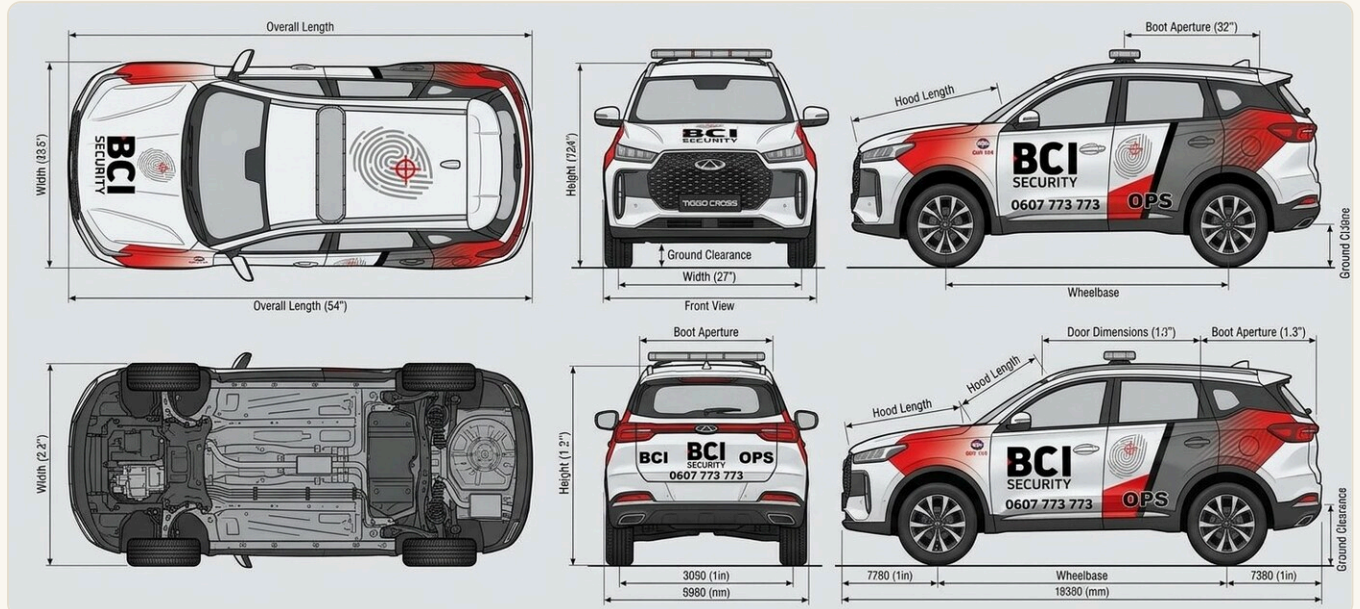
FULL BCI LIVERY SHOWN ACROSS EVERY ANGLE · TOP, FRONT, REAR AND PROFILE · LIGHT BAR AND UNIT IDENTIFIERS TO SPECIFICATION
