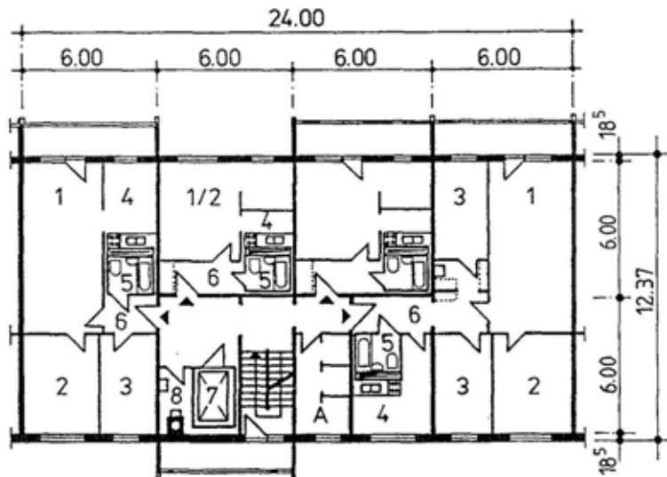
Mittelsegment, Normalgeschoß (1. - 7./9. OG)
